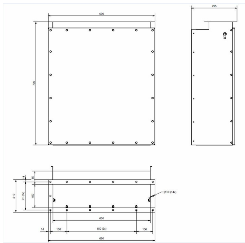
Outlet connection OSF 500FC / OMF 1000FC
